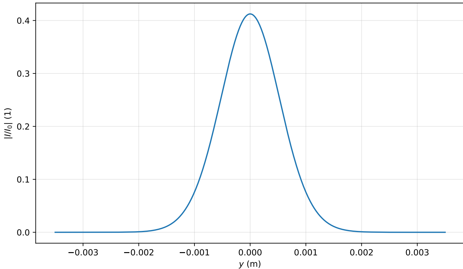
Intensity profile I(x=0, y, z=2.786)/I_0 , P_{in}=0.2P_{cr} , artificial time
